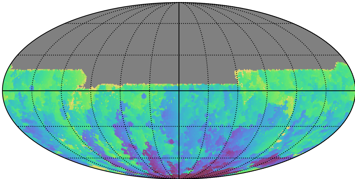
no_high_blob_v3.3_10yrs All sky u band: Min HA
