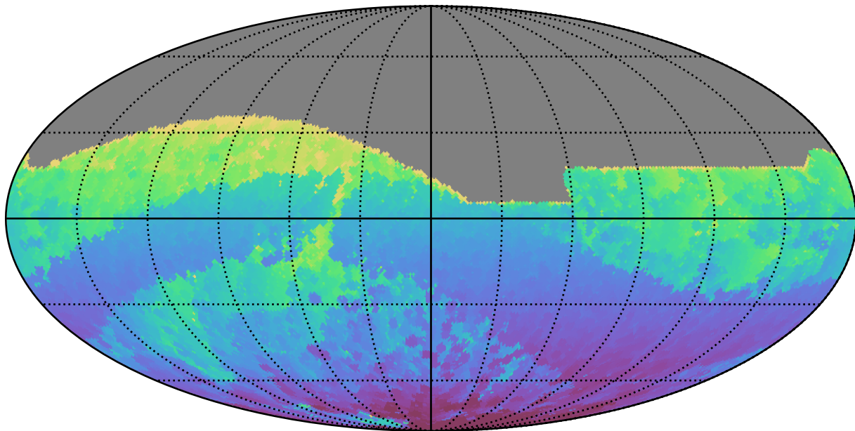
no_high_blob_v3.3_10yrs All sky r band: Min HA
