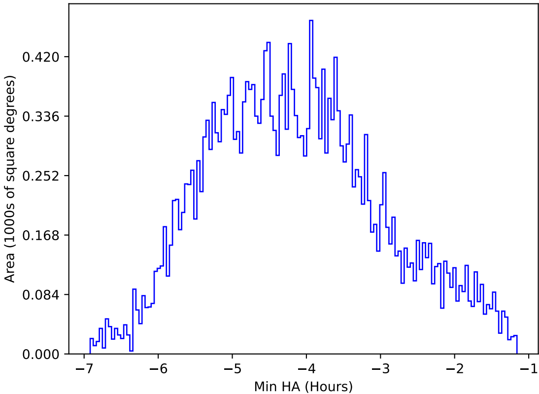
no_high_blob_v3.3_10yrs All sky r band: Min HA
