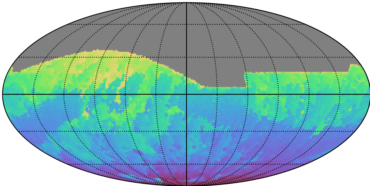
no_high_blob_v3.3_10yrs All sky i band: Min HA
