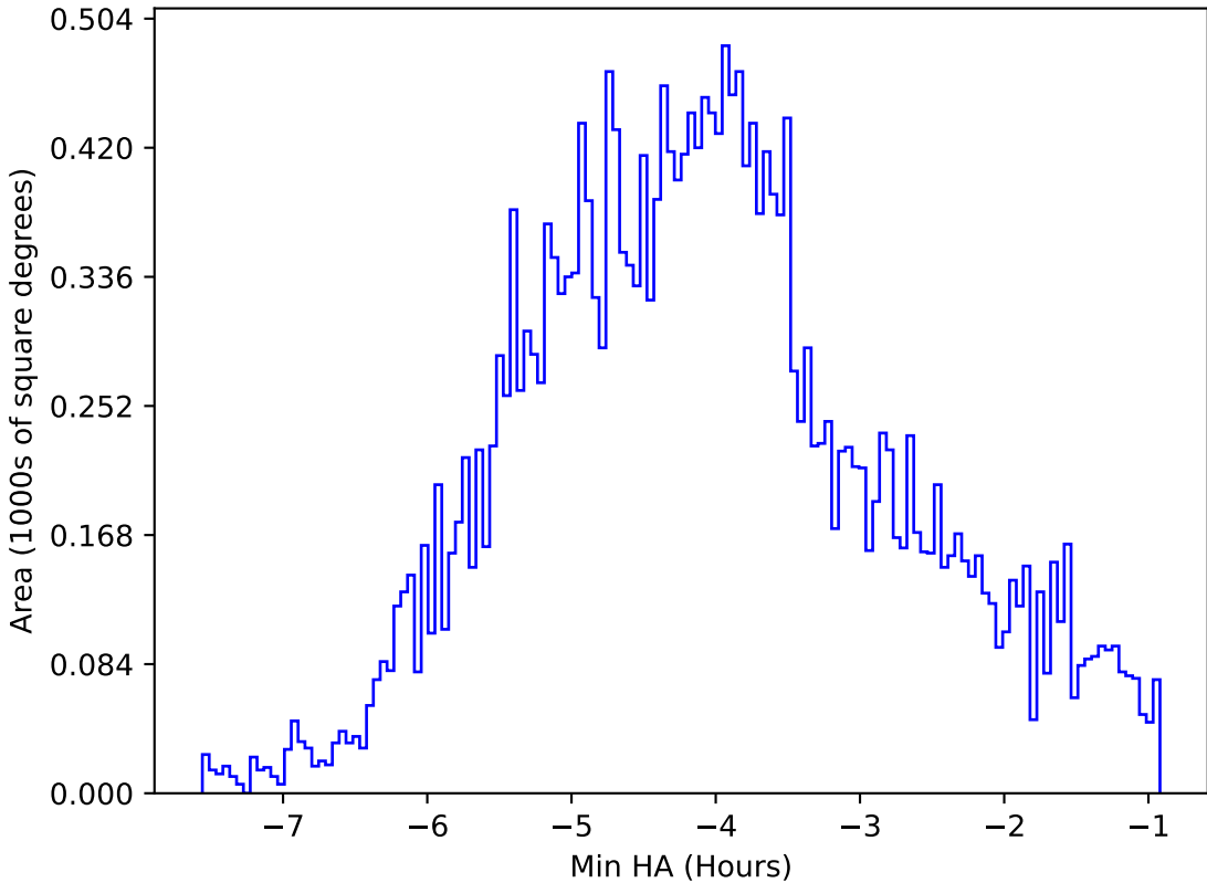
no_high_blob_v3.3_10yrs All sky i band: Min HA
