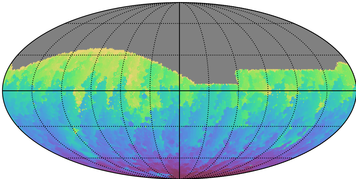
no_high_blob_v3.3_10yrs All sky g band: Min HA
