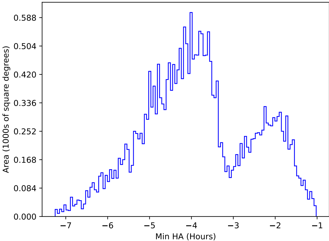
no_high_blob_v3.3_10yrs All sky g band: Min HA
