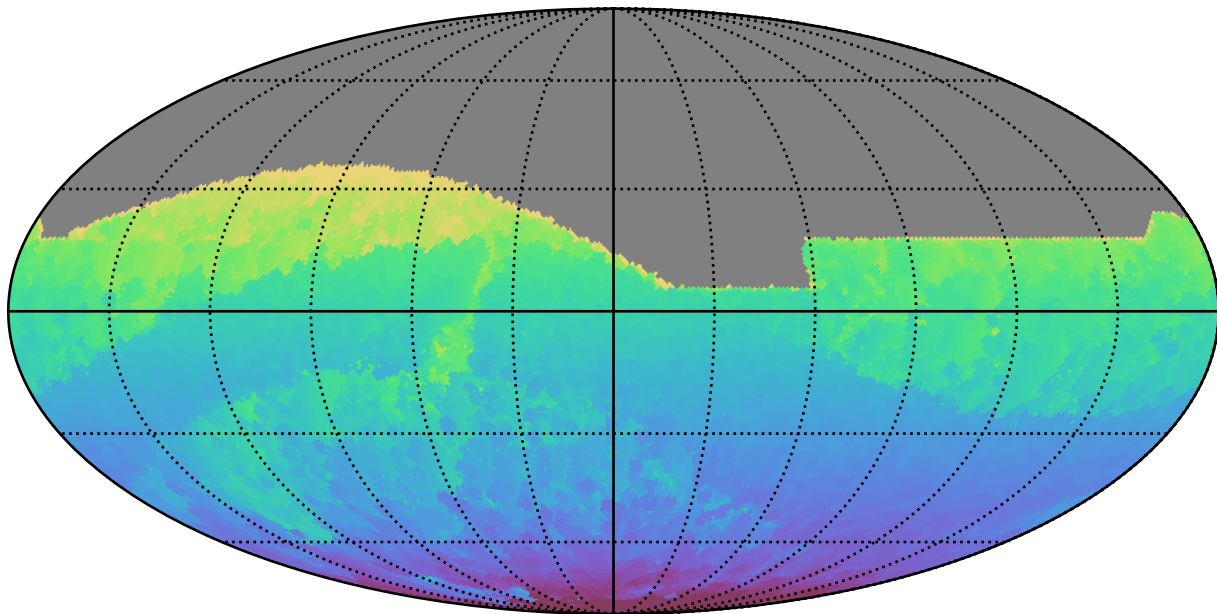
no_high_blob_v3.3_10yrs All sky all bands: Min HA
