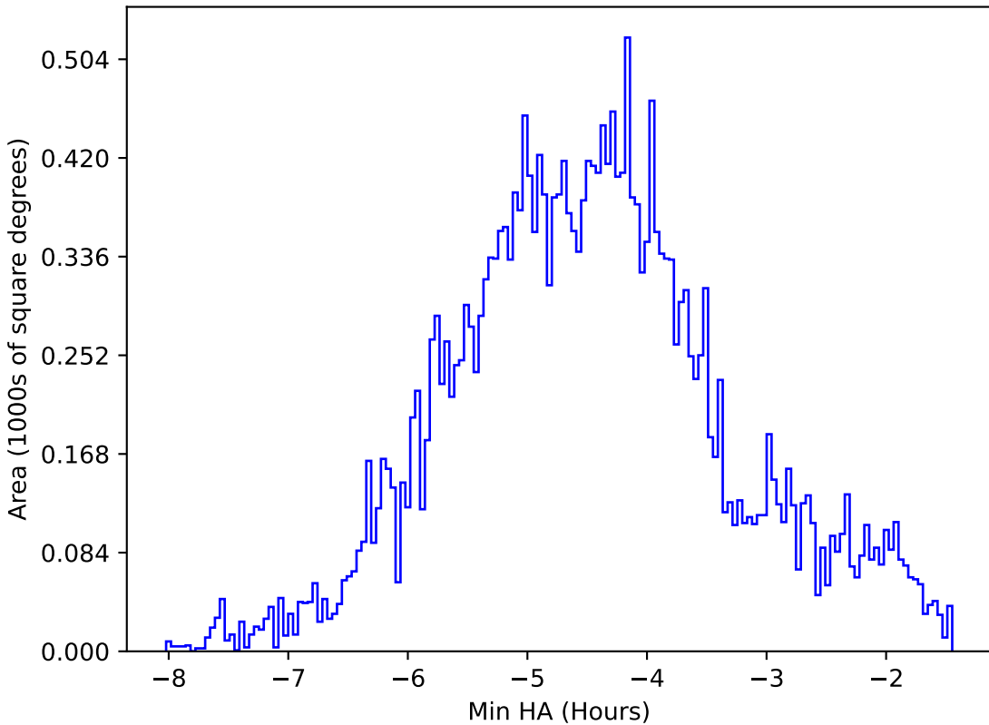
no_high_blob_v3.3_10yrs All sky all bands: Min HA
