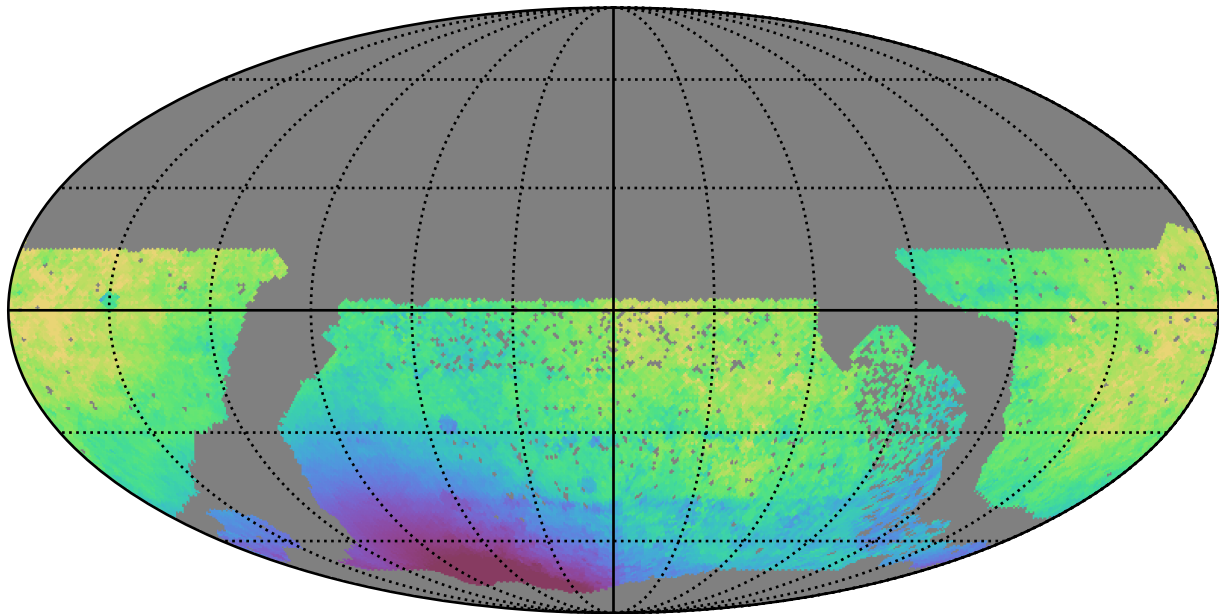
no_high_blob_v3.3_10yrs WFD z band: Median solarElong
