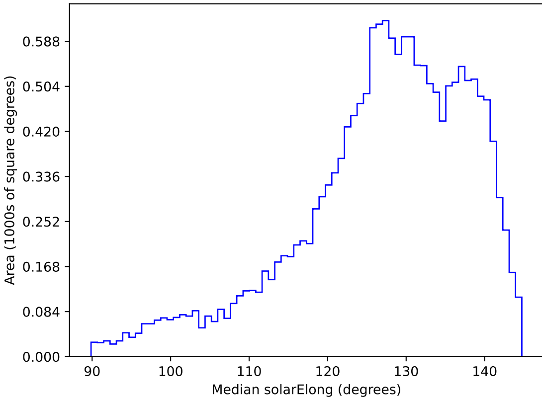
no_high_blob_v3.3_10yrs WFD z band: Median solarElong
