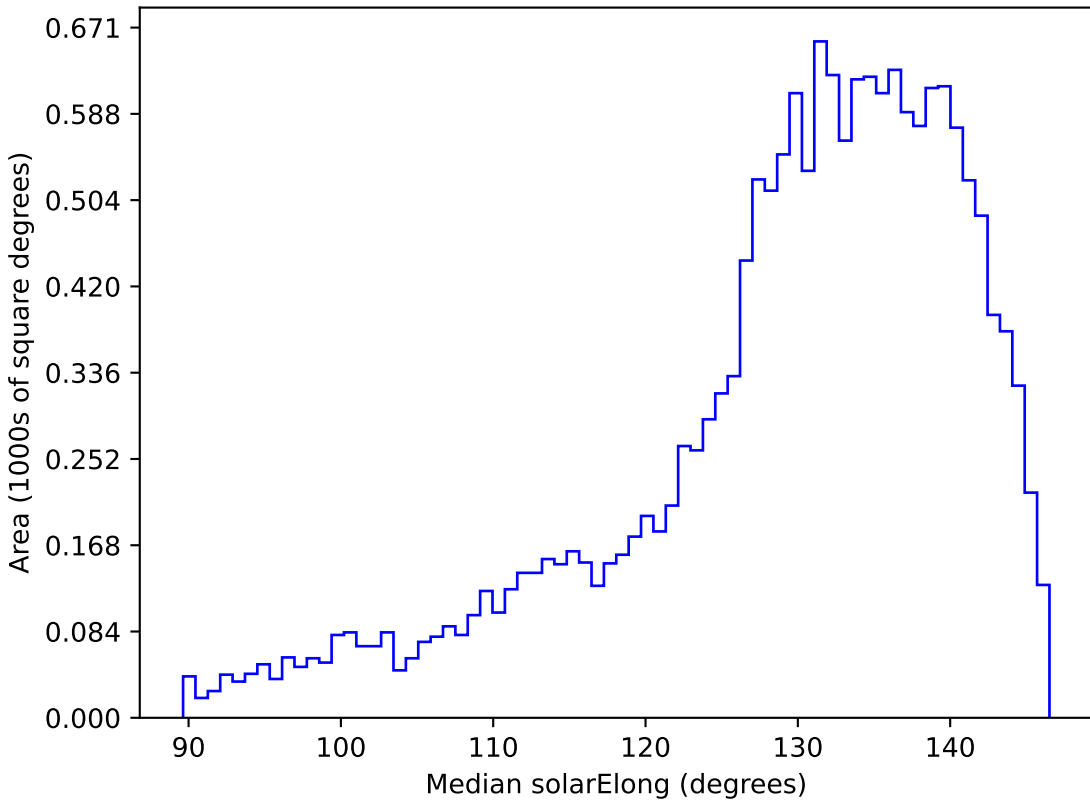
no_high_blob_v3.3_10yrs WFD y band: Median solarElong
