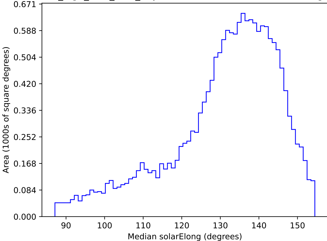
no_high_blob_v3.3_10yrs WFD u band: Median solarElong
