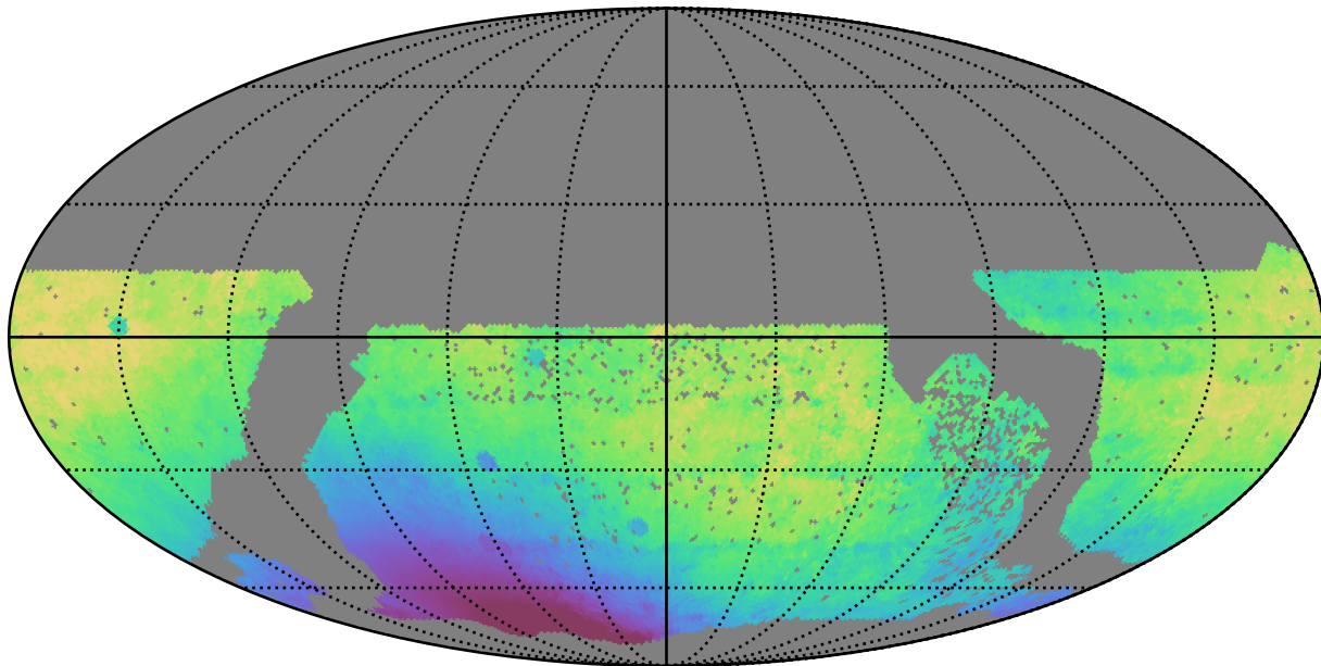
no_high_blob_v3.3_10yrs WFD r band: Median solarElong
