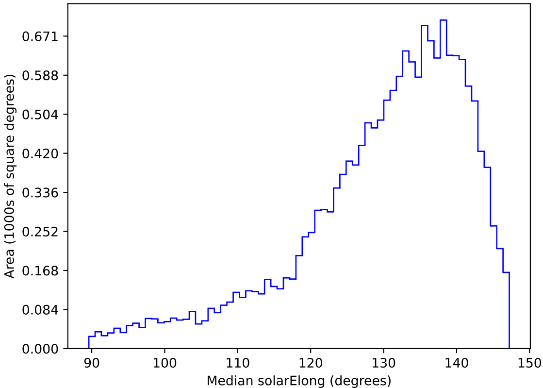
no_high_blob_v3.3_10yrs WFD r band: Median solarElong
