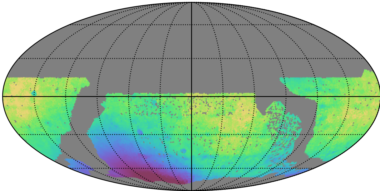
no_high_blob_v3.3_10yrs WFD i band: Median solarElong
