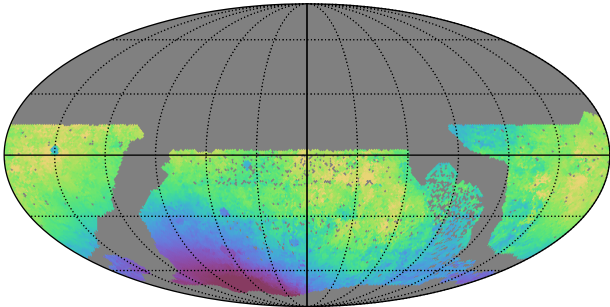
no_high_blob_v3.3_10yrs WFD g band: Median solarElong
