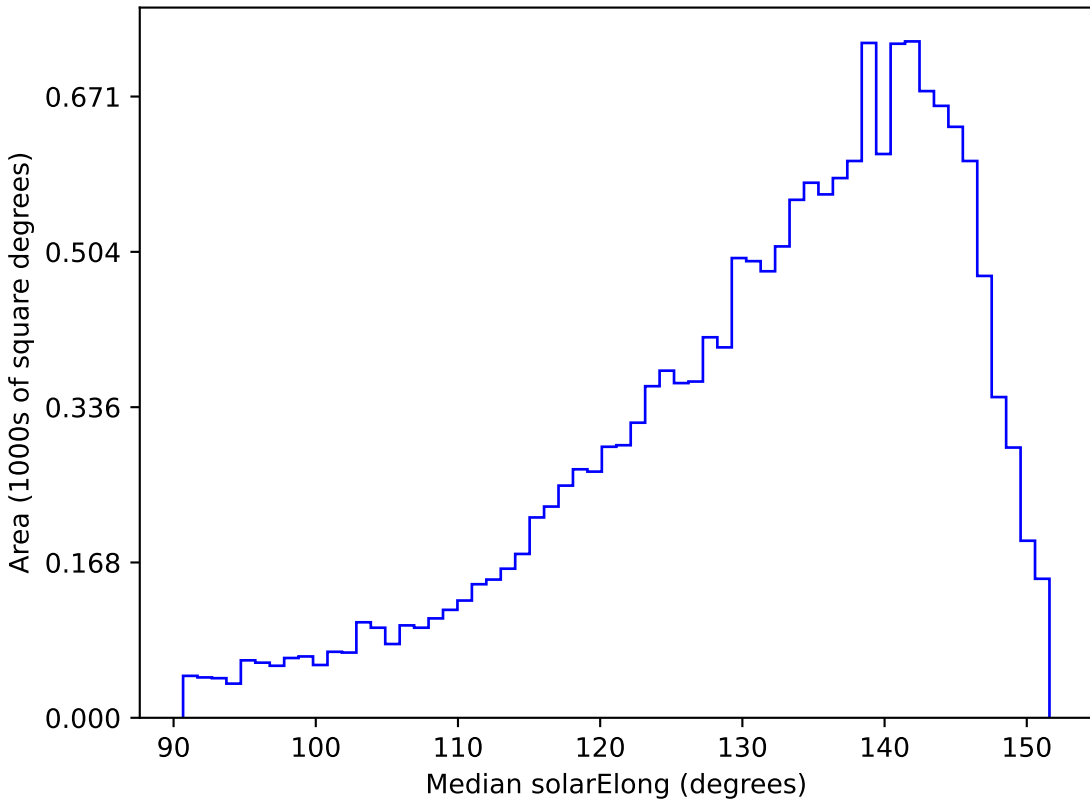
no_high_blob_v3.3_10yrs WFD g band: Median solarElong
