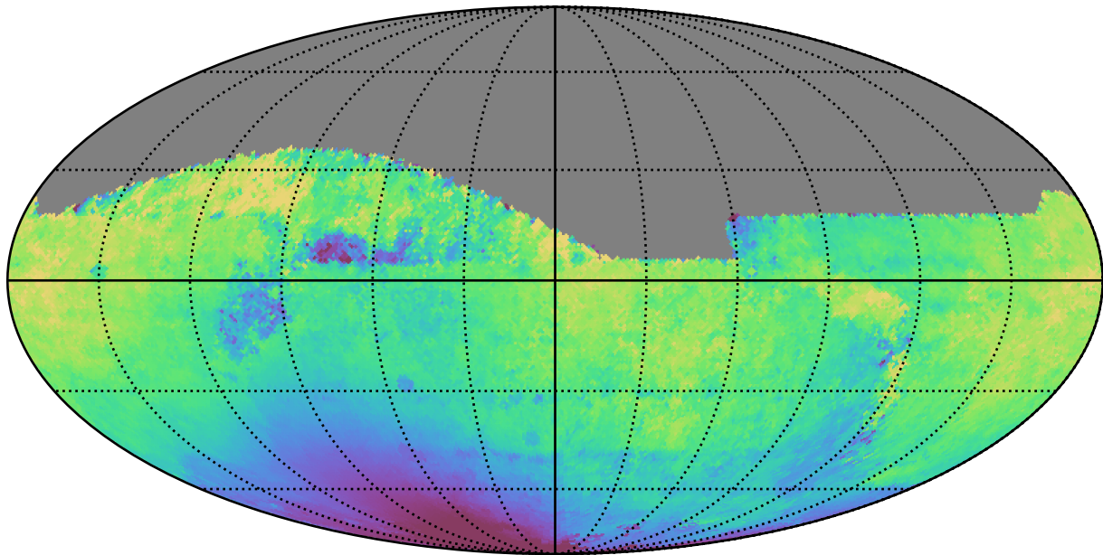
no_high_blob_v3.3_10yrs All sky z band: Median solarElong
