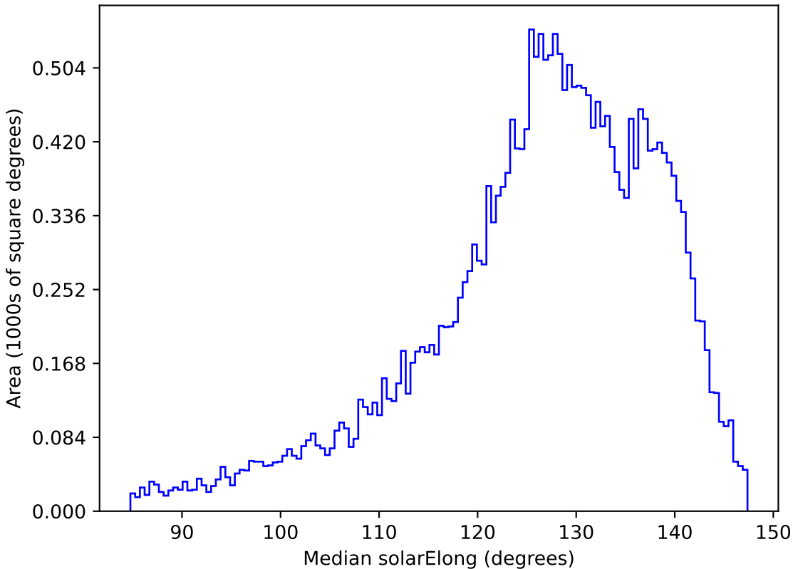
no_high_blob_v3.3_10yrs All sky z band: Median solarElong
