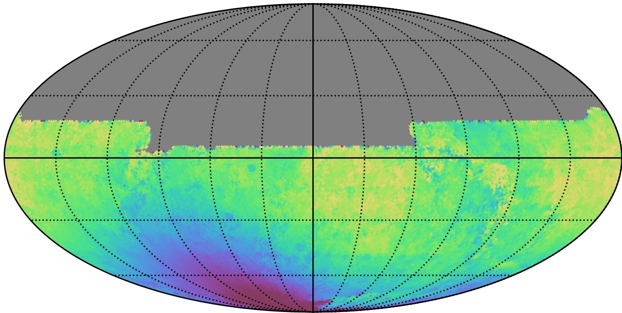
no_high_blob_v3.3_10yrs All sky y band: Median solarElong
