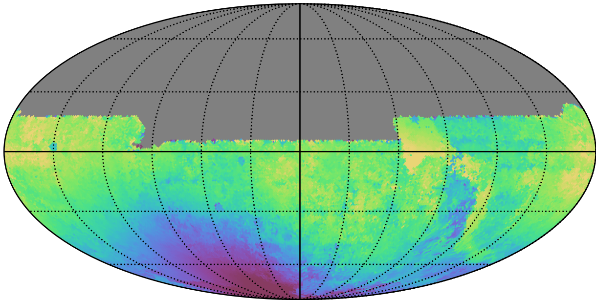
no_high_blob_v3.3_10yrs All sky u band: Median solarElong
