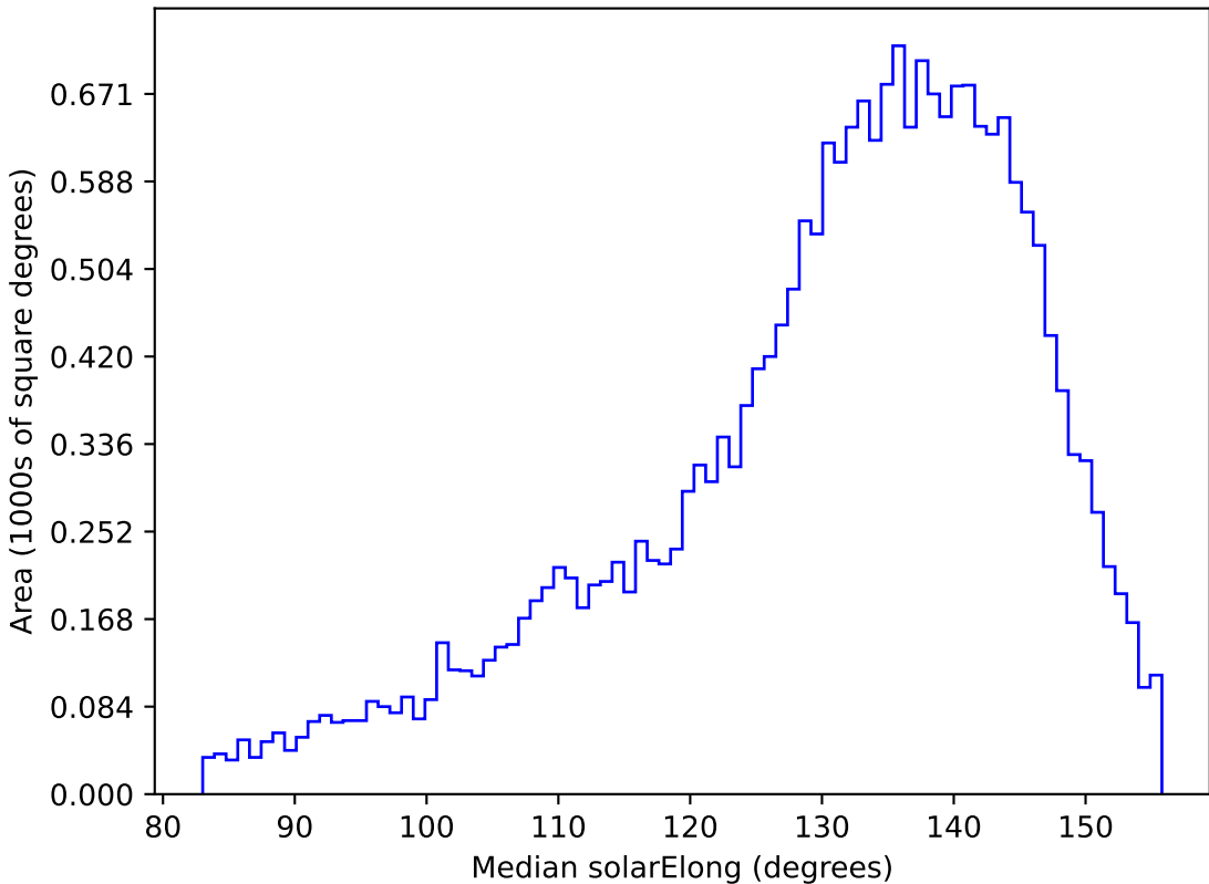
no_high_blob_v3.3_10yrs All sky u band: Median solarElong
