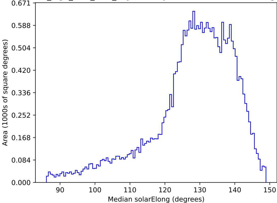
no_high_blob_v3.3_10yrs All sky i band: Median solarElong
