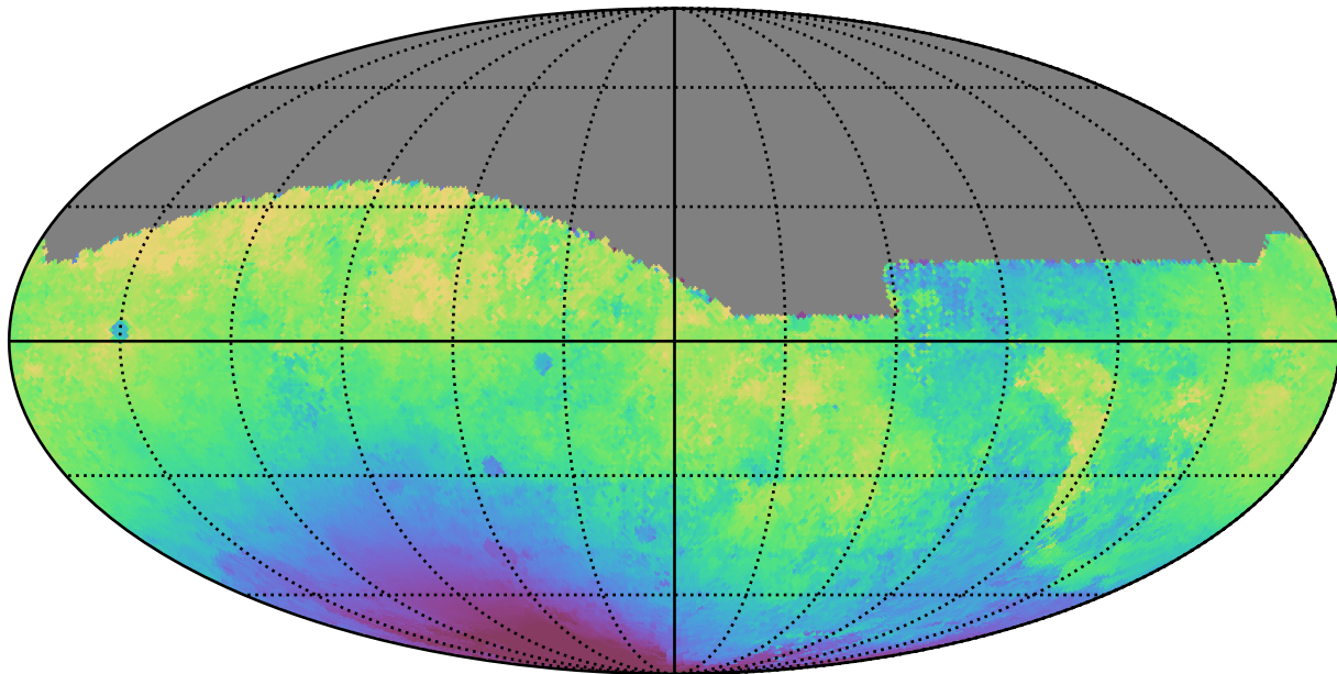
no_high_blob_v3.3_10yrs All sky g band: Median solarElong
