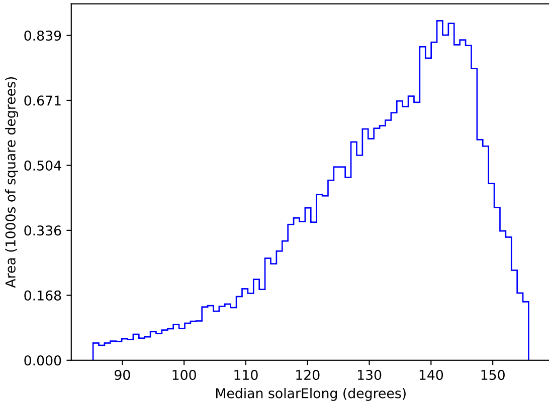
no_high_blob_v3.3_10yrs All sky g band: Median solarElong
