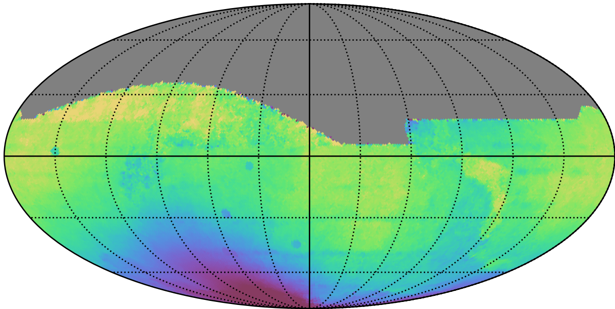
no_high_blob_v3.3_10yrs All sky all bands: Median solarElong
