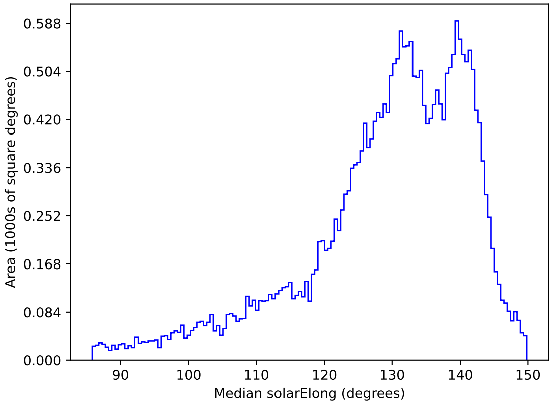
no_high_blob_v3.3_10yrs All sky all bands: Median solarElong
