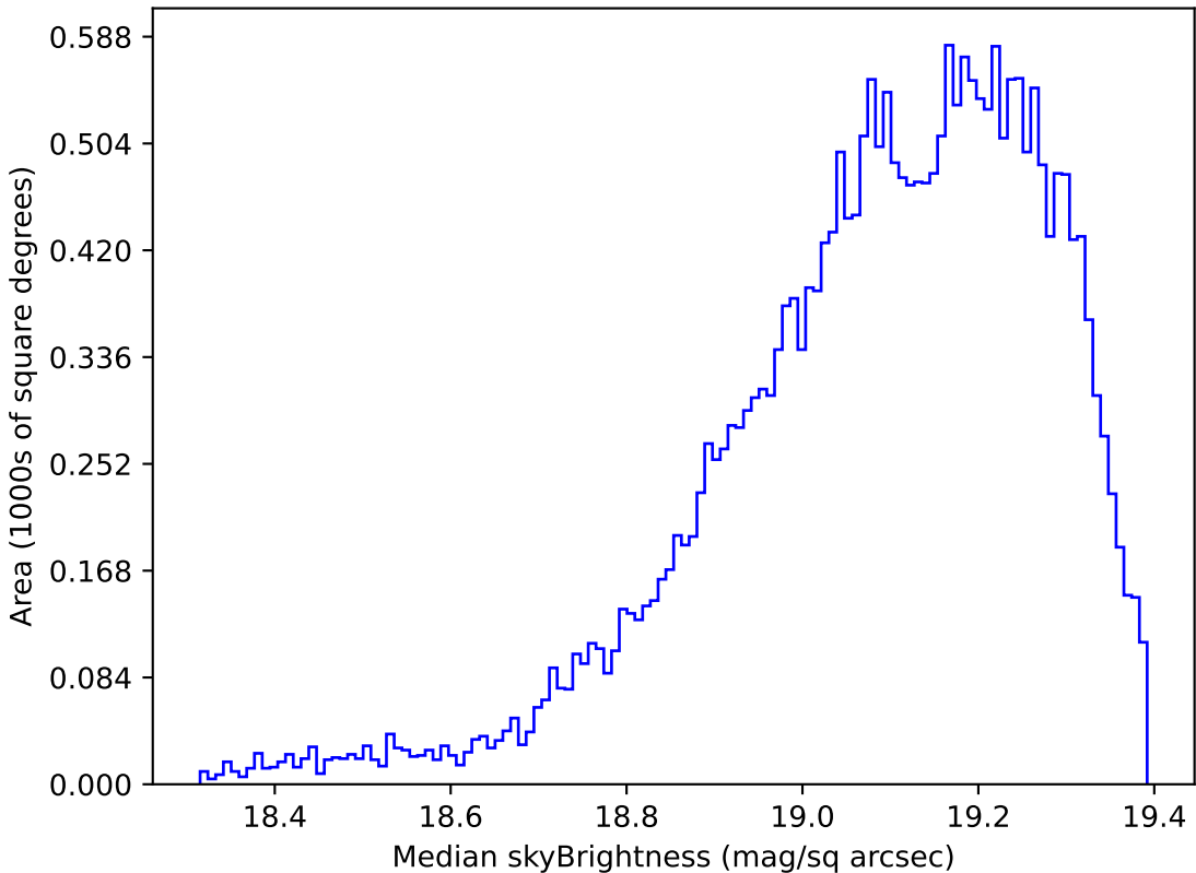
no_high_blob_v3.3_10yrs Yr 1 z band: Median skyBrightness
