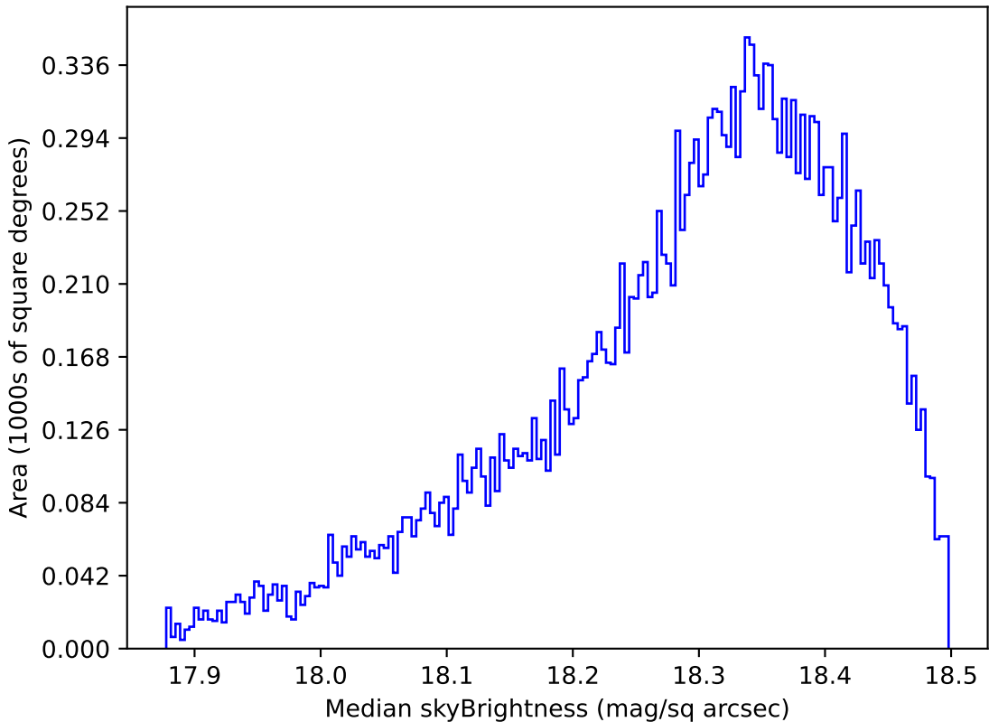
no_high_blob_v3.3_10yrs Yr 1 y band: Median skyBrightness
