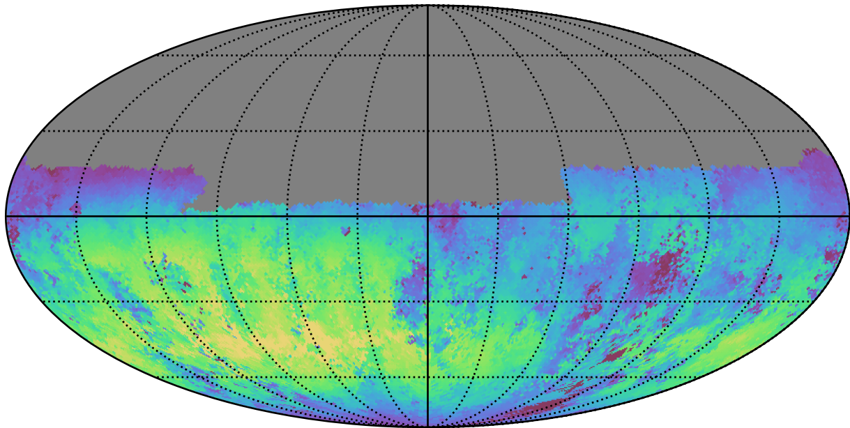
no_high_blob_v3.3_10yrs Yr 1 u band: Median skyBrightness
