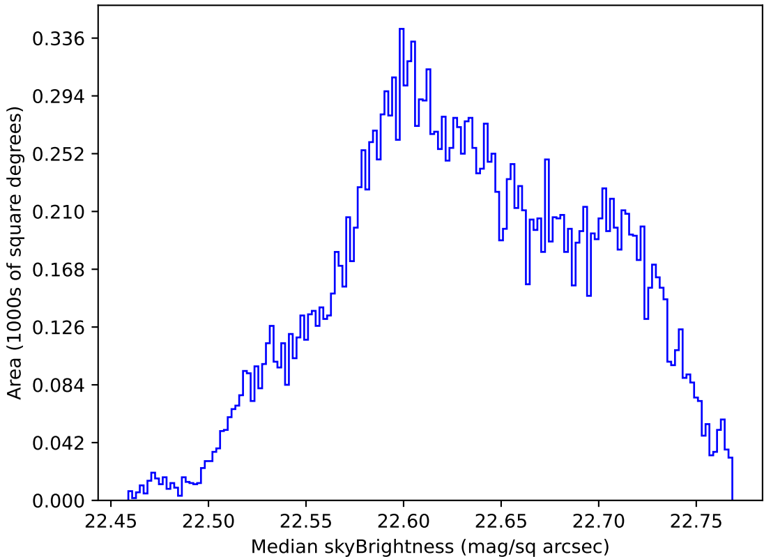
no_high_blob_v3.3_10yrs Yr 1 u band: Median skyBrightness
