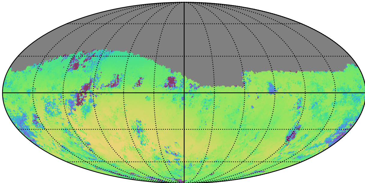
no_high_blob_v3.3_10yrs Yr 1 r band: Median skyBrightness
