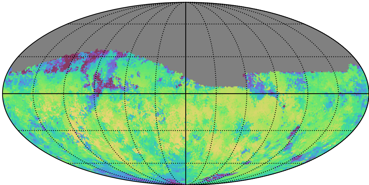
no_high_blob_v3.3_10yrs Yr 1 i band: Median skyBrightness
