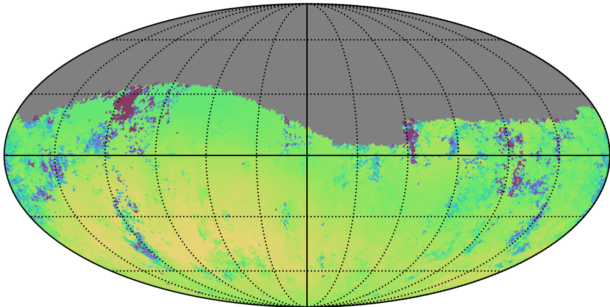
no_high_blob_v3.3_10yrs Yr 1 g band: Median skyBrightness
