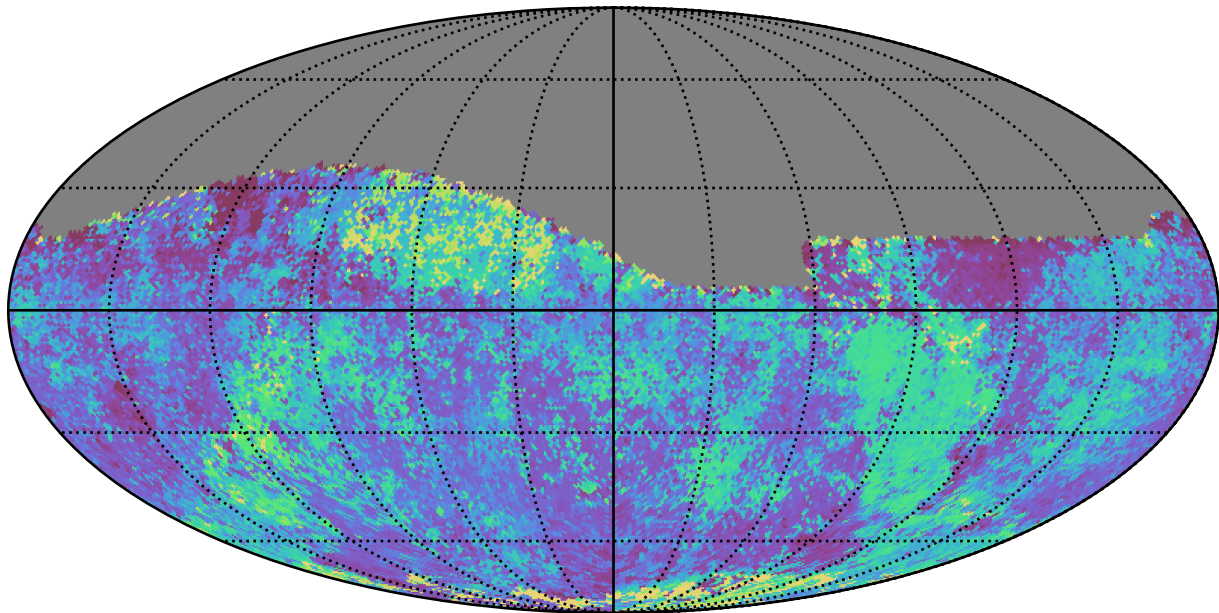
no_high_blob_v3.3_10yrs Yr 1 all bands: Median skyBrightness
