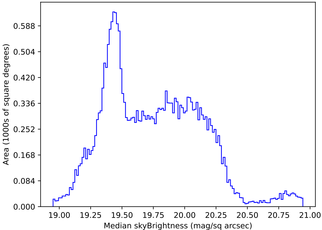
no_high_blob_v3.3_10yrs Yr 1 all bands: Median skyBrightness
