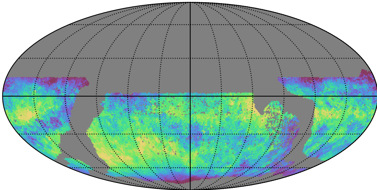
no_high_blob_v3.3_10yrs WFD z band: Median skyBrightness
