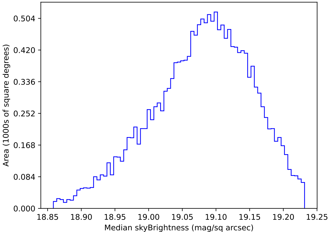
no_high_blob_v3.3_10yrs WFD z band: Median skyBrightness
