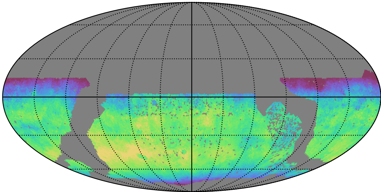
no_high_blob_v3.3_10yrs WFD y band: Median skyBrightness
