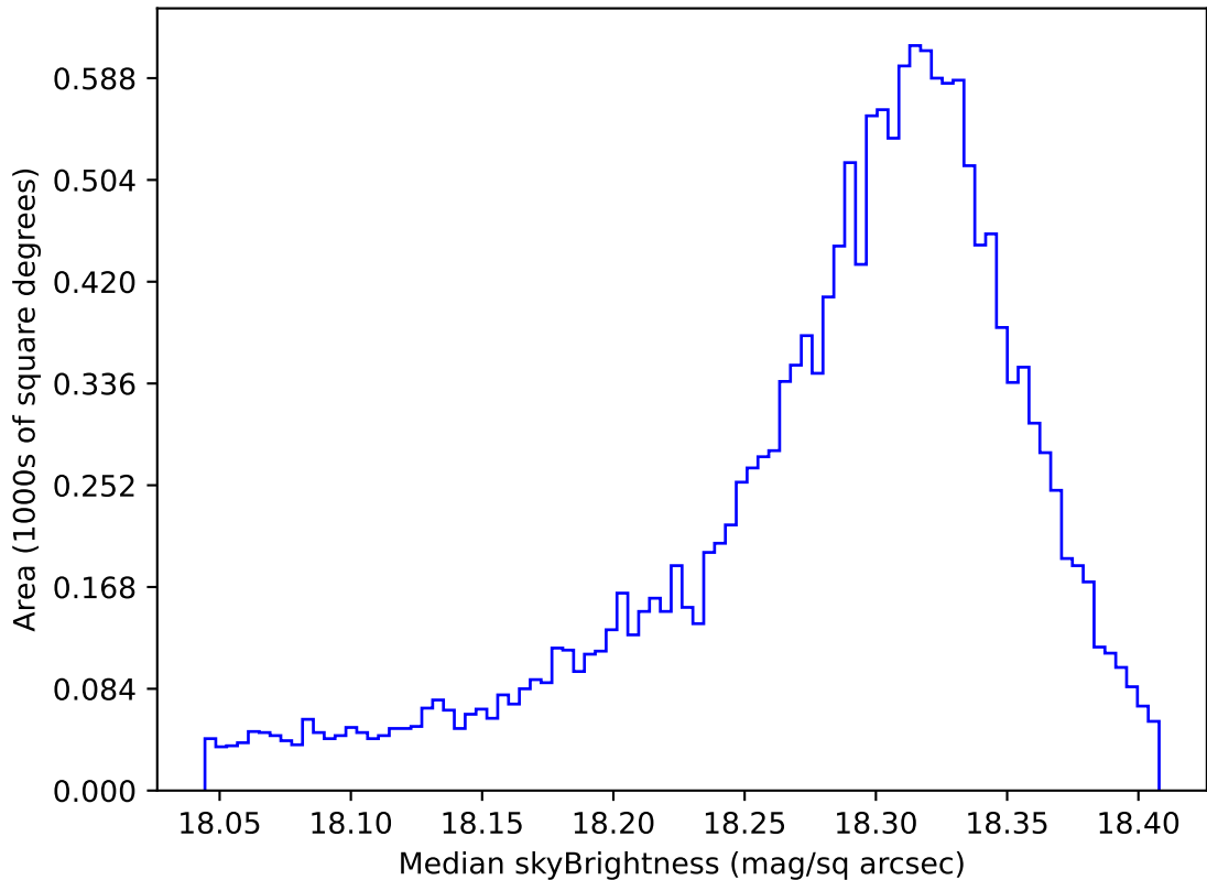
no_high_blob_v3.3_10yrs WFD y band: Median skyBrightness
