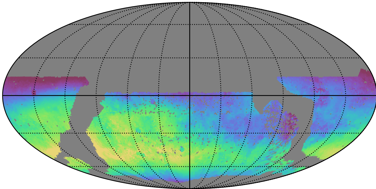
no_high_blob_v3.3_10yrs WFD u band: Median skyBrightness
