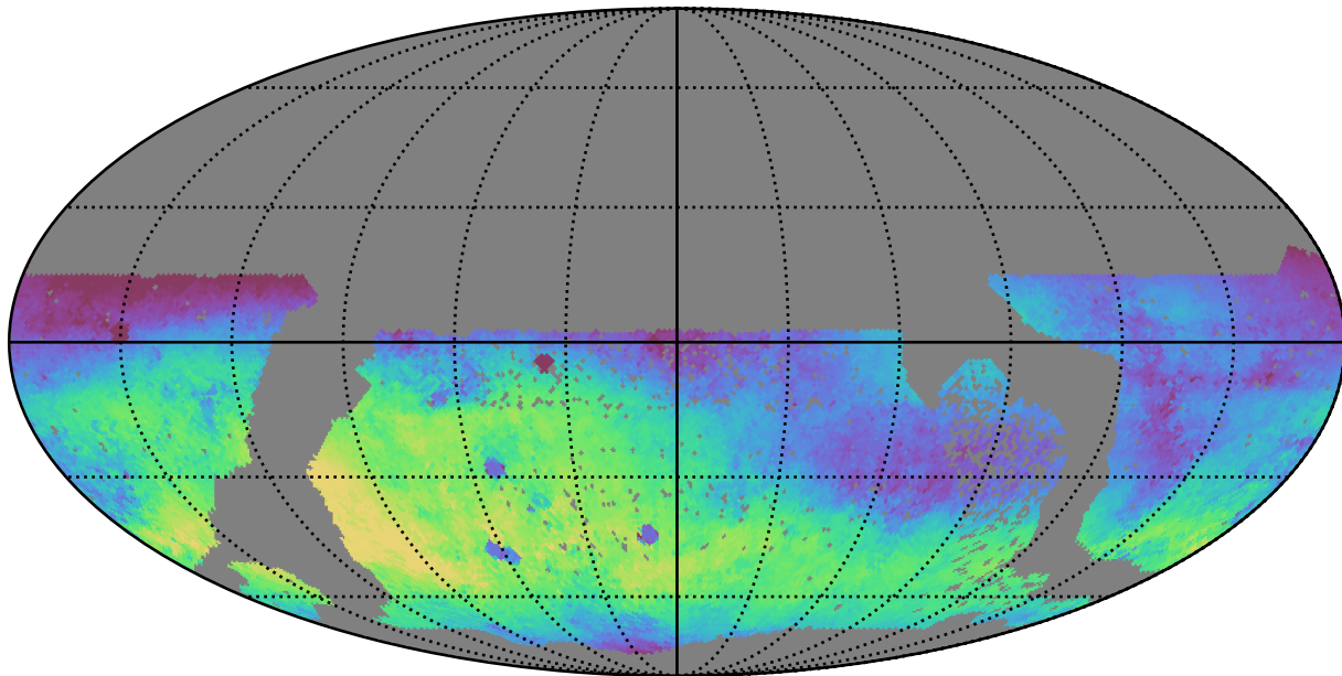
no_high_blob_v3.3_10yrs WFD r band: Median skyBrightness
