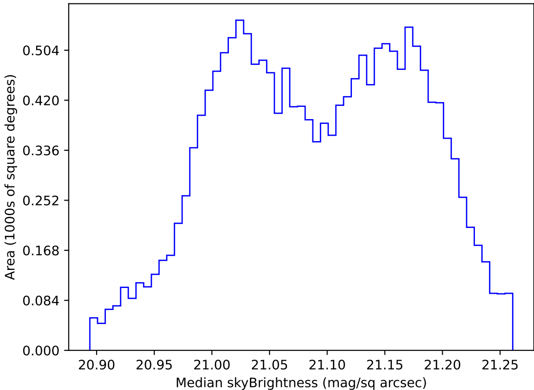
no_high_blob_v3.3_10yrs WFD r band: Median skyBrightness
