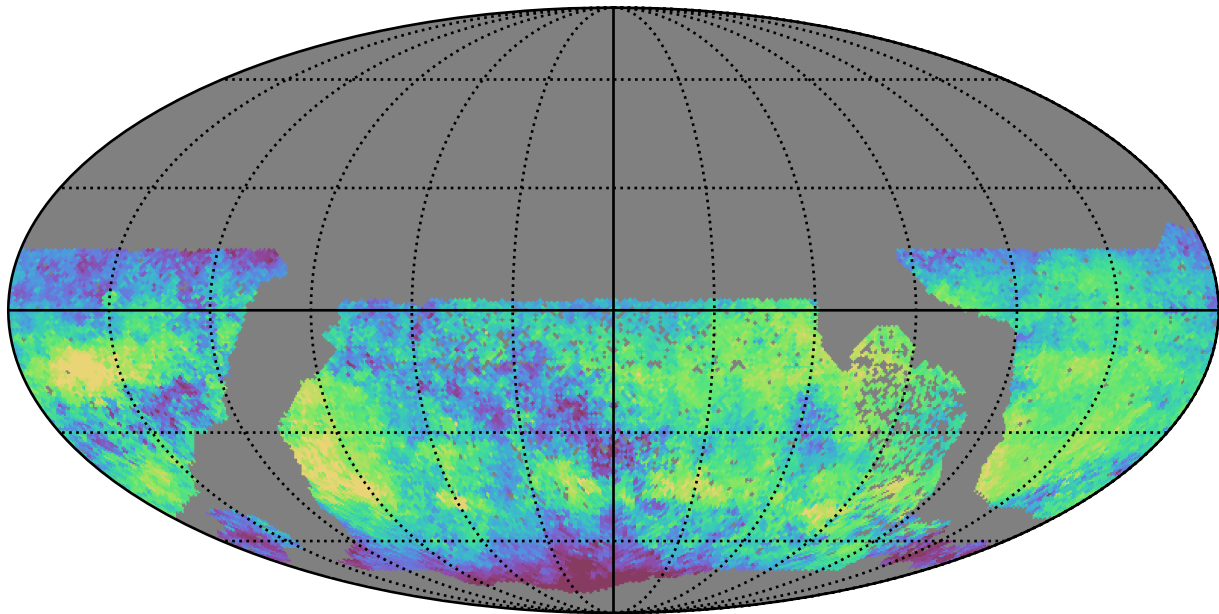
no_high_blob_v3.3_10yrs WFD i band: Median skyBrightness
