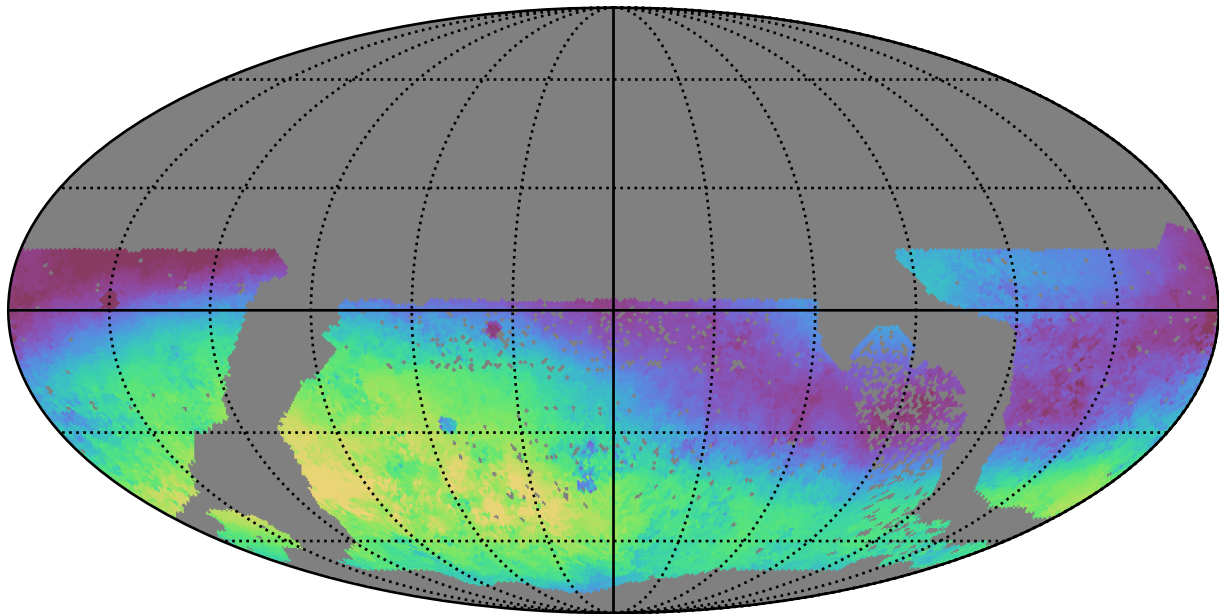
no_high_blob_v3.3_10yrs WFD g band: Median skyBrightness
