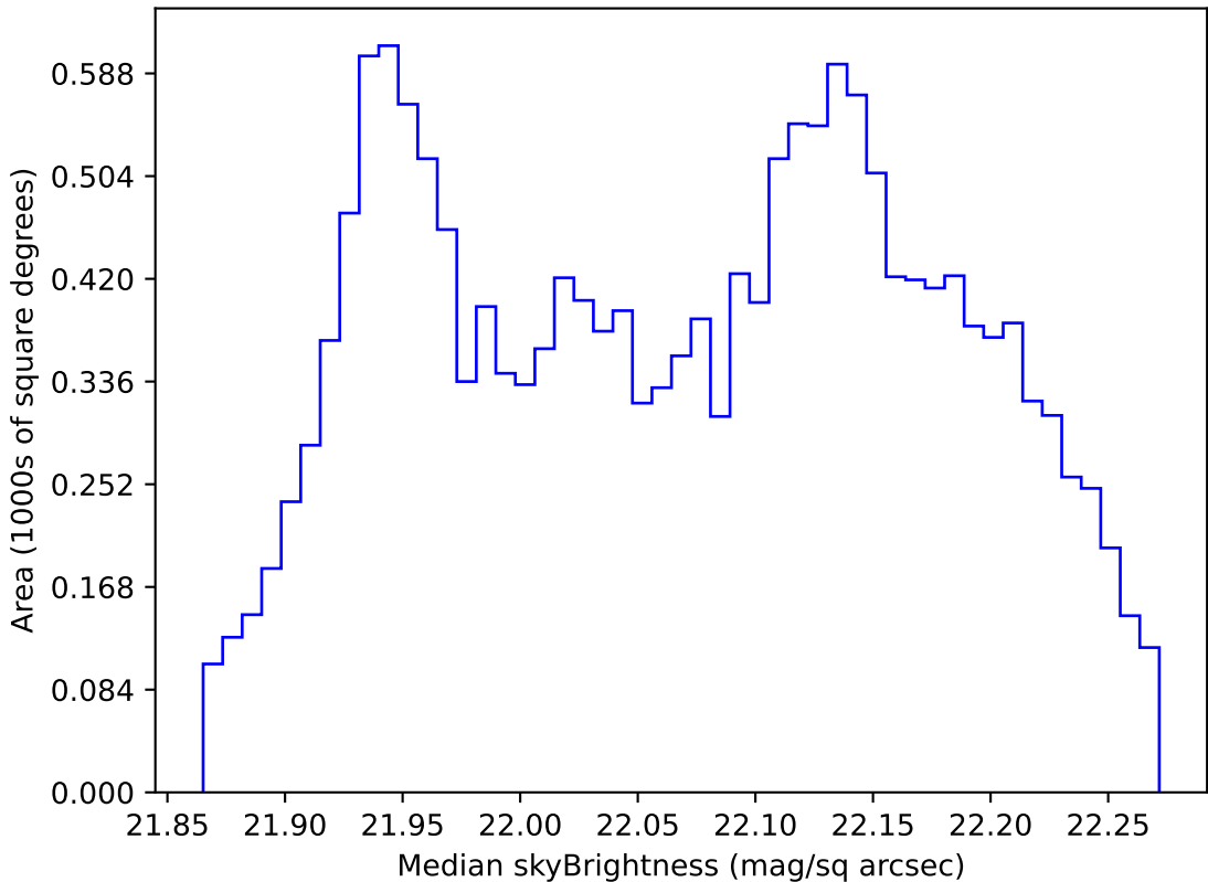
no_high_blob_v3.3_10yrs WFD g band: Median skyBrightness
