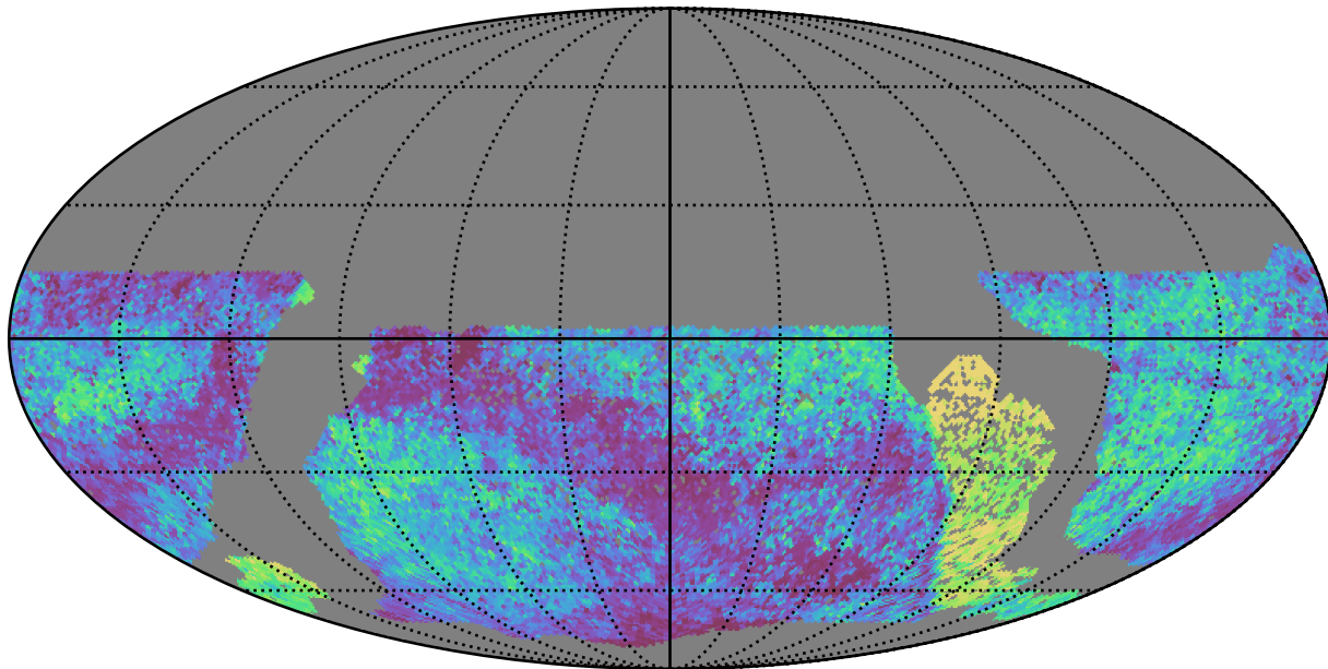
no_high_blob_v3.3_10yrs WFD all bands: Median skyBrightness
