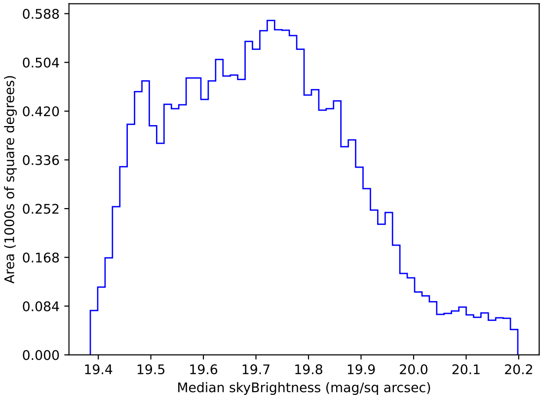
no_high_blob_v3.3_10yrs WFD all bands: Median skyBrightness
