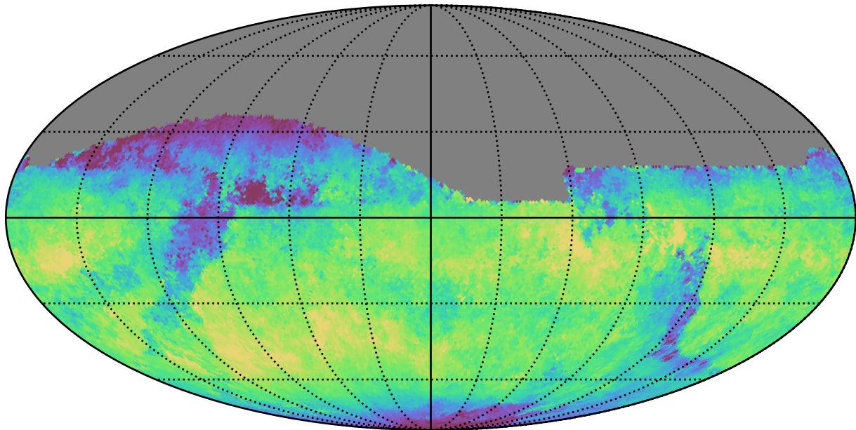
no_high_blob_v3.3_10yrs All sky z band: Median skyBrightness
